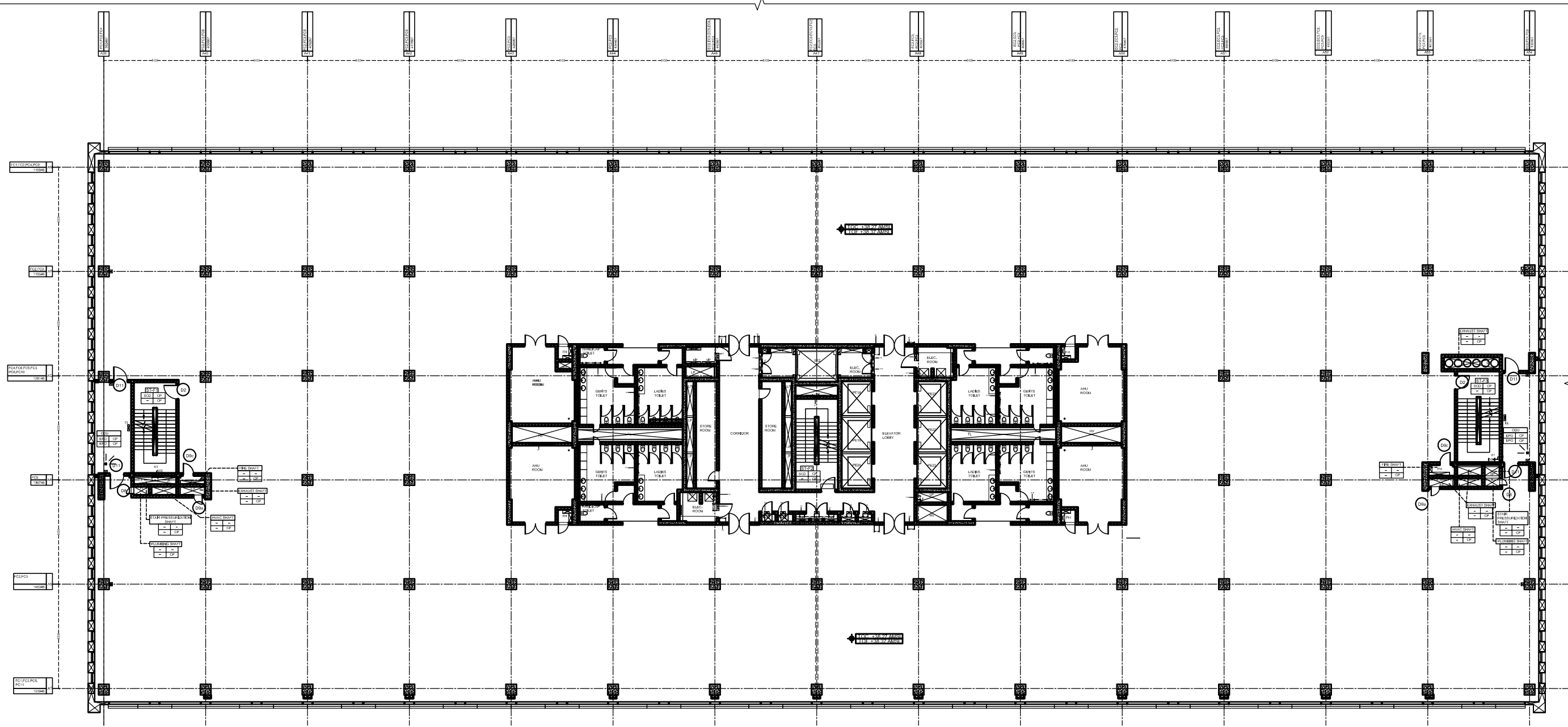
1. TYPICAL FLOOR WORKING PLAN - BLOCK F
